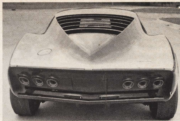
REAR-ON view shows Venetian-blind rear window, pop-open gas filler, retracted stabilizer flaps. Bumper bar also retracts into body.
