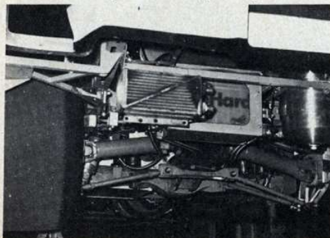
Race car's rear suspension has unequal-length A-arms.
